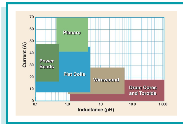
Fig. 1 Current and inductance characteristics of the various types of power inductors.
